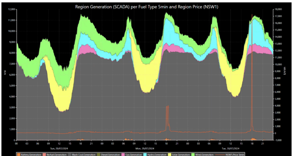
Figure 25 Price Impacts from High Renewable Energy (New South Wales)
