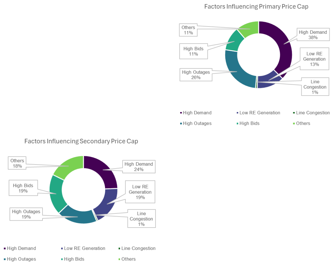
Figure 23 Price Driver Frequency Split between PPC and SPC (5-minute Market)
