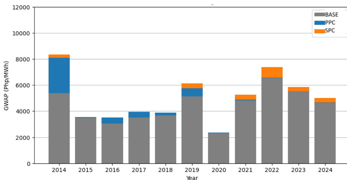
Figure 18 Luzon Historical Annual Average GWAP
