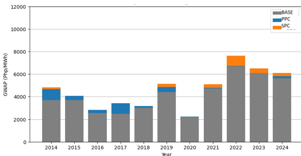
Figure 19 Visayas Historical Annual Average GWAP
