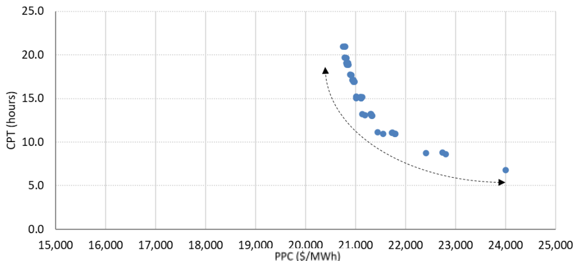
Figure 7 Possible combinations of the primary price cap and secondary price cap
