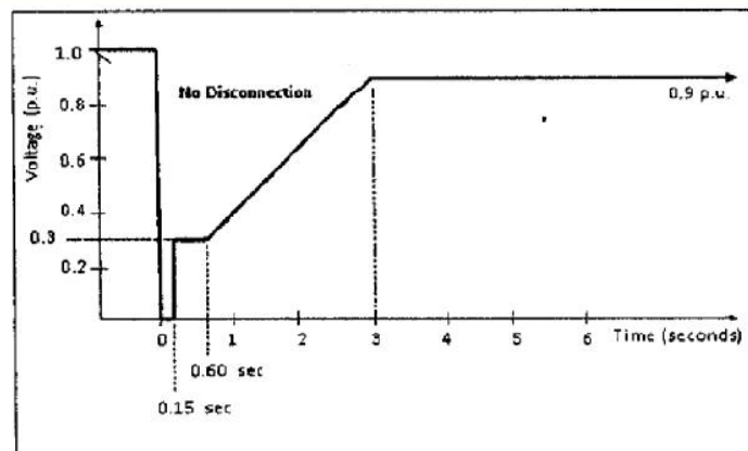
Figure 4: Low voltage withstand capability – PVS
